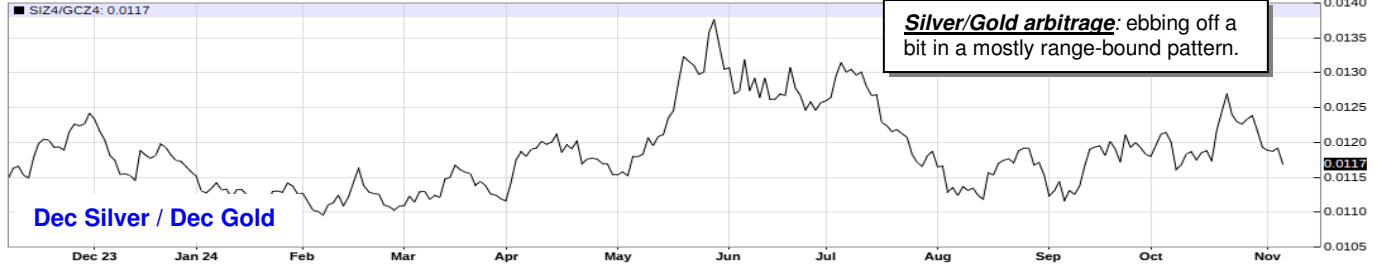
SIZ24/GCZ24 - Spread Chart
