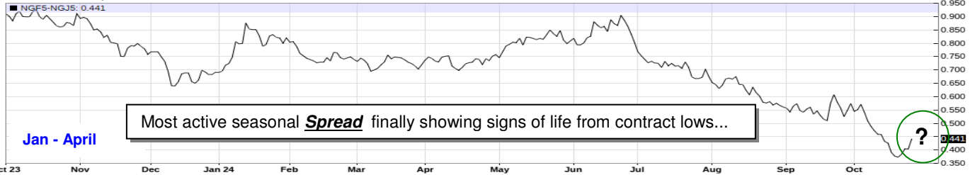
NGF25-NGJ25 - Spread Chart
