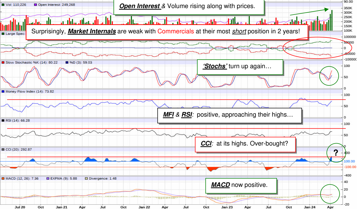
RM - Robusta Coffee 10-T - Weekly Nearest Candlestick Chart
