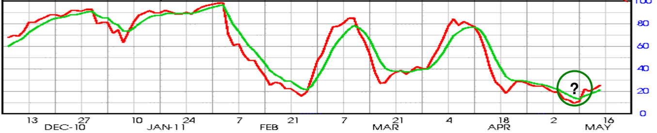
SUGAR #11 OCT 2011 ... daily Stochastic - %k and %d 14 3
