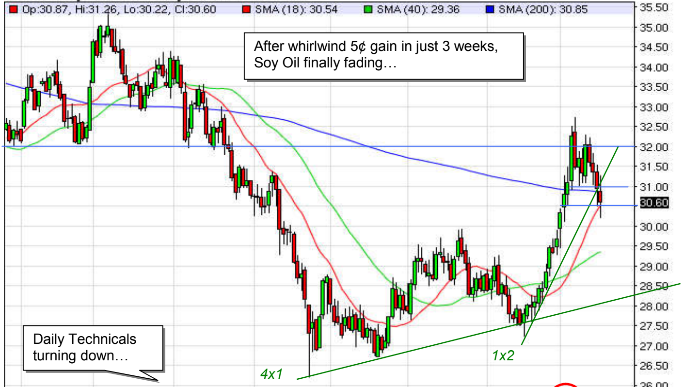
ZLH16 - Soybean Oil - Daily Candlestick Chart
