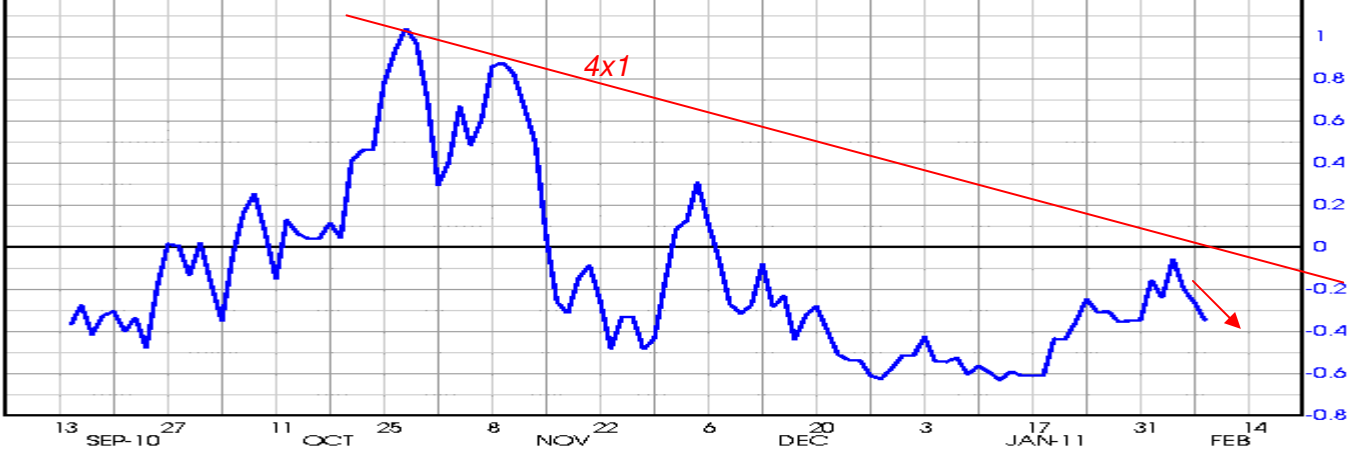
RRK11 RRX11 spread ... daily Close only plot
