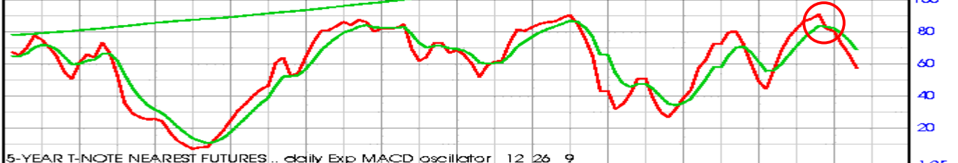
5-YEAR T-NOTE NEAREST FUTURES... daily Exp MACD oscillator 12 26 9
