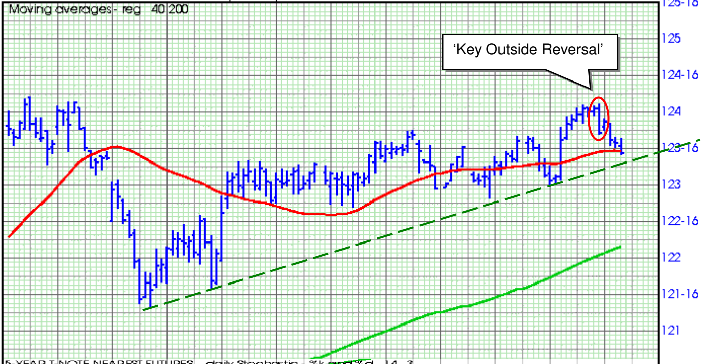
5-YEAR T-NOTE NEAREST FUTURES... daily Stochastic - %k and %d 14 3
