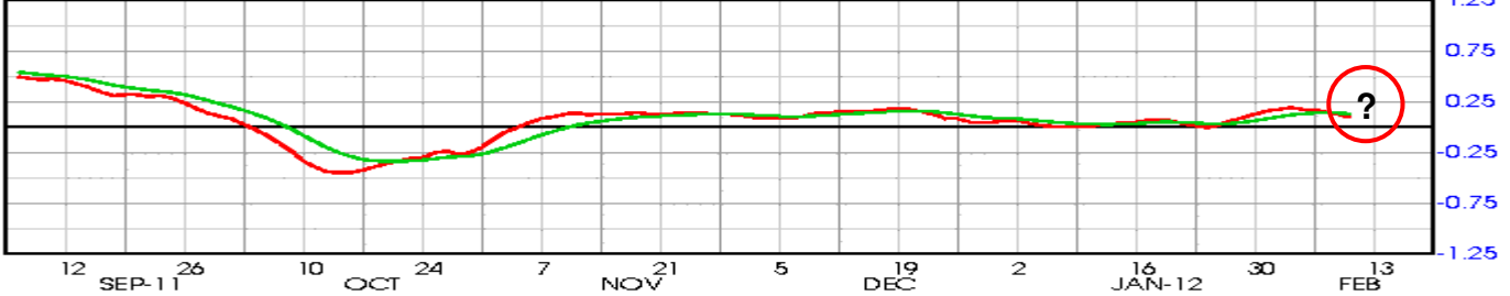
5-YEAR T-NOTE NEAREST FUTURES... daily Exp MACD oscillator 12 26 9
